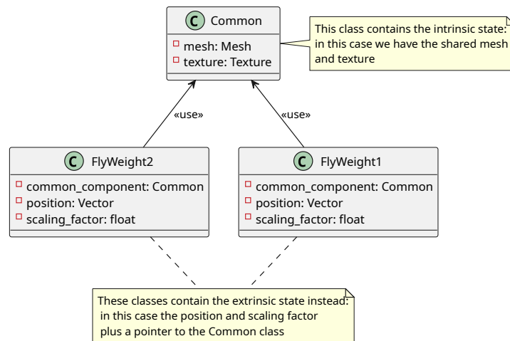
Figure 311: UML Diagram of the Flyweight pattern
